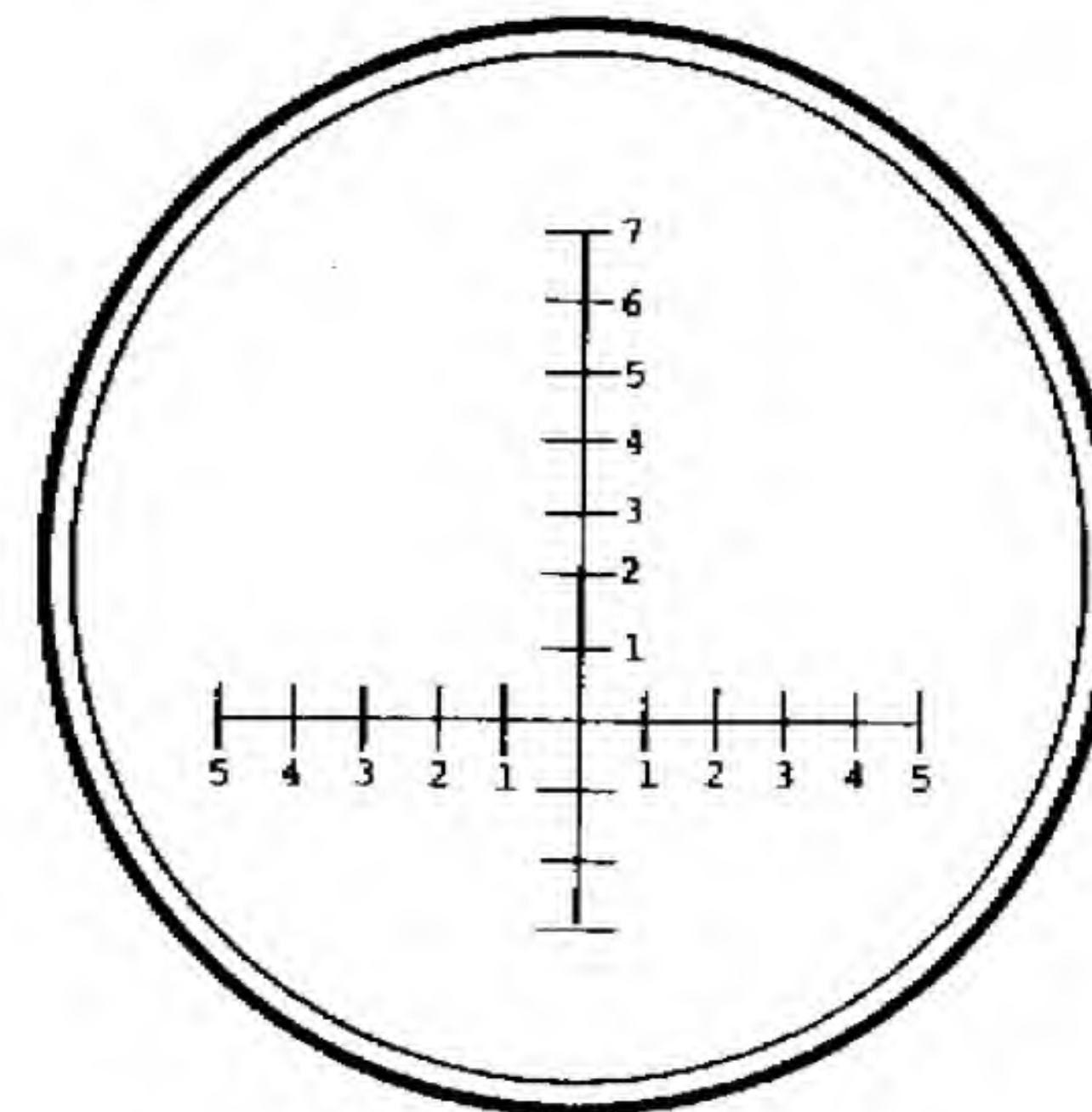
Figure 2-27. M19 reticle.
