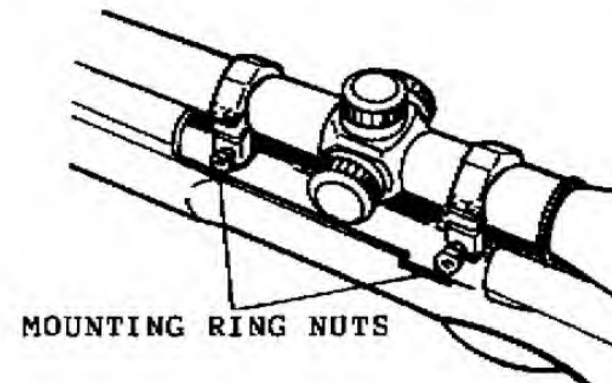
Figure 2-8. Ring nuts.
